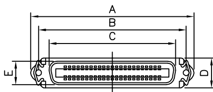
Male (With Straight Metal cover)
