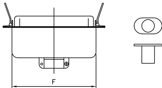
Female (With Straight Metal cover)
