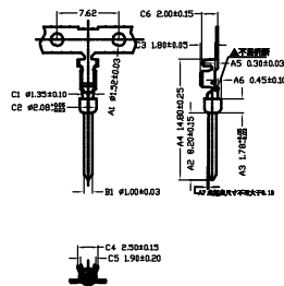
CRIMP High feet male terminal
