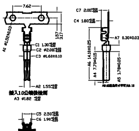
CRIMP High feet female terminal
