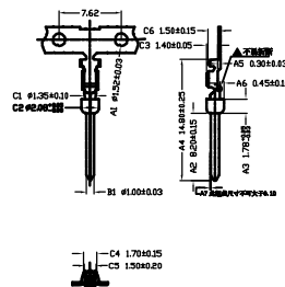
CRIMP Low feet male terminal
