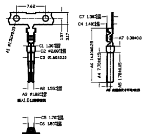
CRIMP Low feet female terminal
